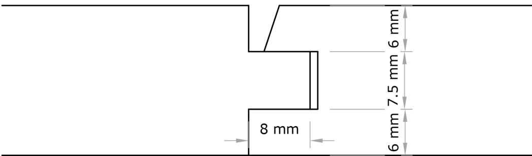
ANGLE SHADOW GAP
