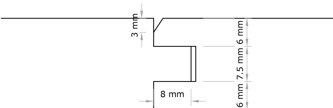
CHAMFER SHADOW GAP
